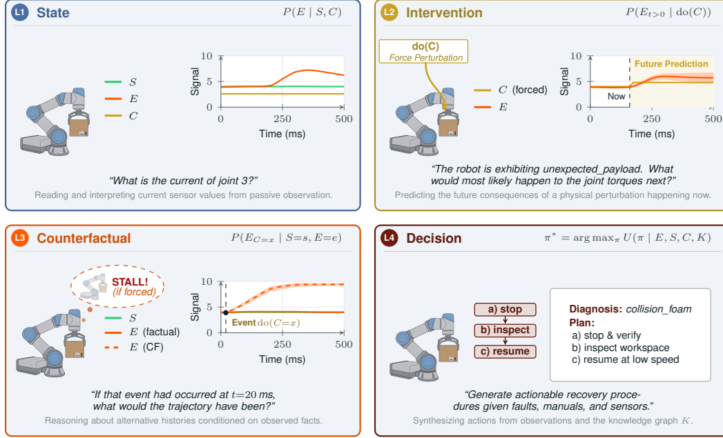
Figure 5: The four levels of machine understanding defined by FactoryBench.
