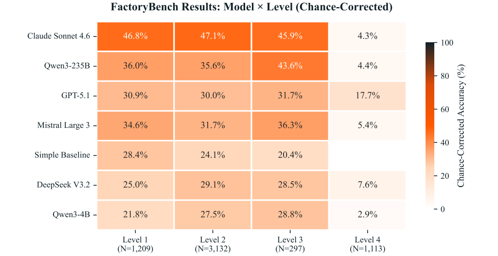
(a) Chance-corrected accuracy (%) on FactoryBench’s four reasoning levels.
