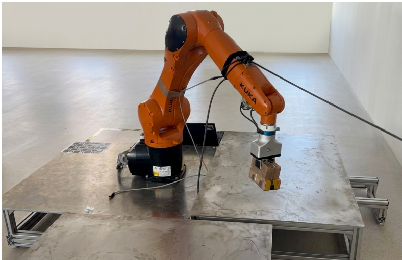
Figure 6: The arm-disturbance fault as physically applied to the KUKA in FactoryWave.
