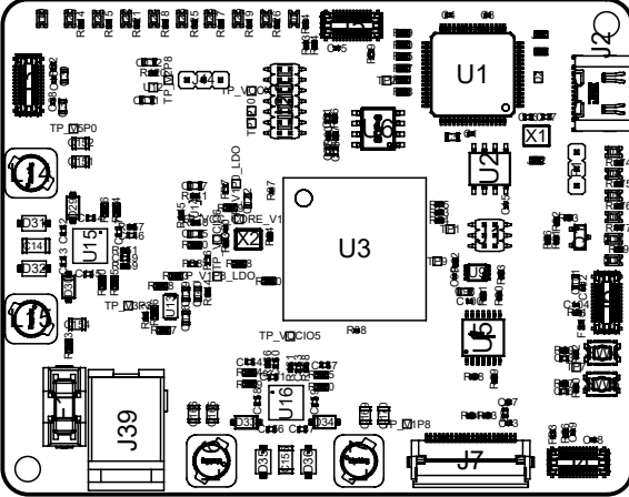
View from Top side (Scale 1:1)
