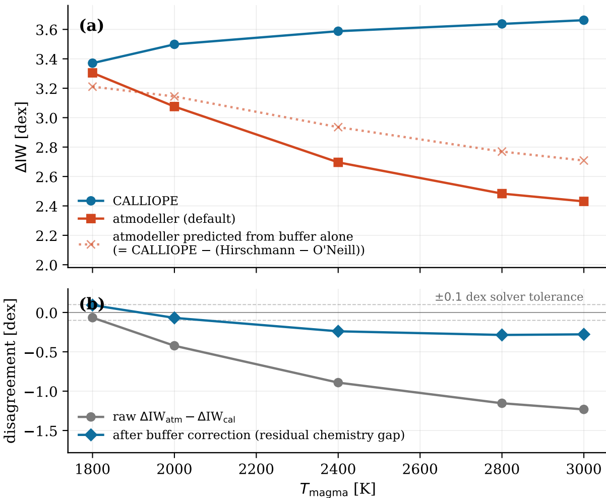
Cross-backend \Delta IW at Earth-BSE volatile inventory, \Phi = 1
