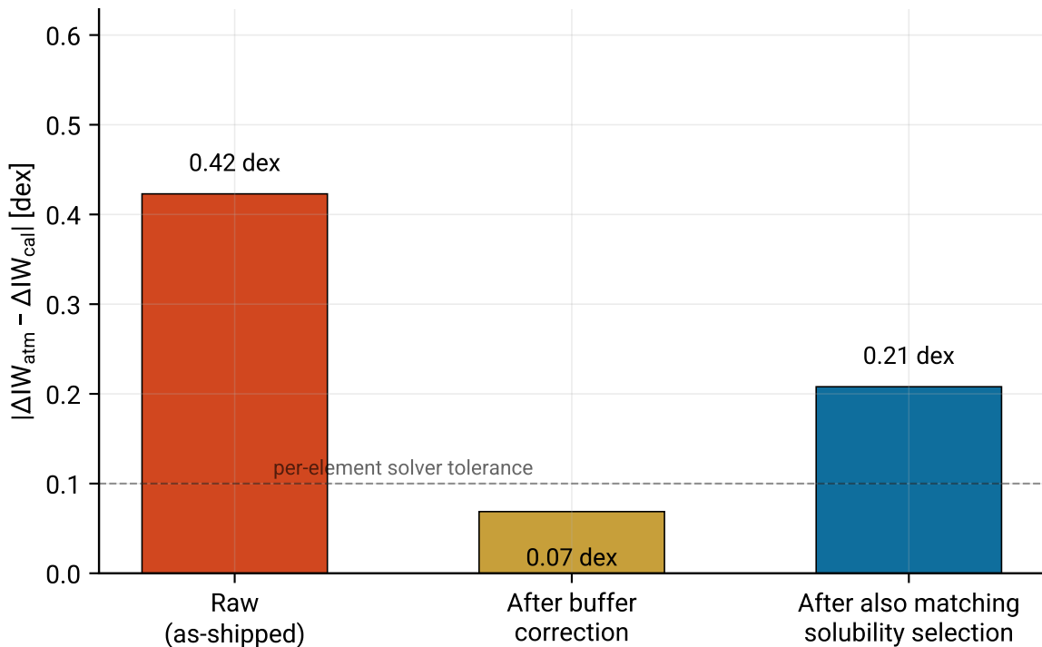
Attribution of cross-backend \Delta IW disagreement at Earth-BSE, T = 2000 K, \Phi = 1
