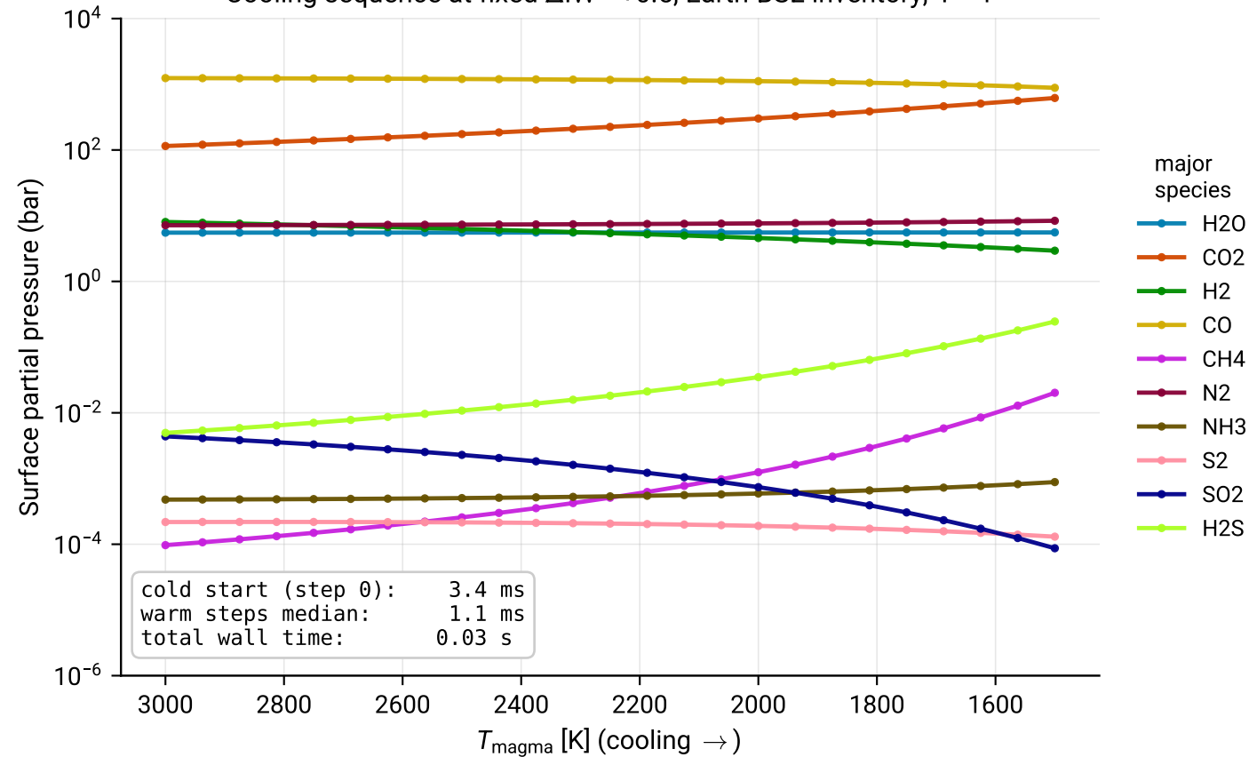
Cooling sequence at fixed \Delta IW = +0.5 , Earth-BSE inventory, \Phi = 1
