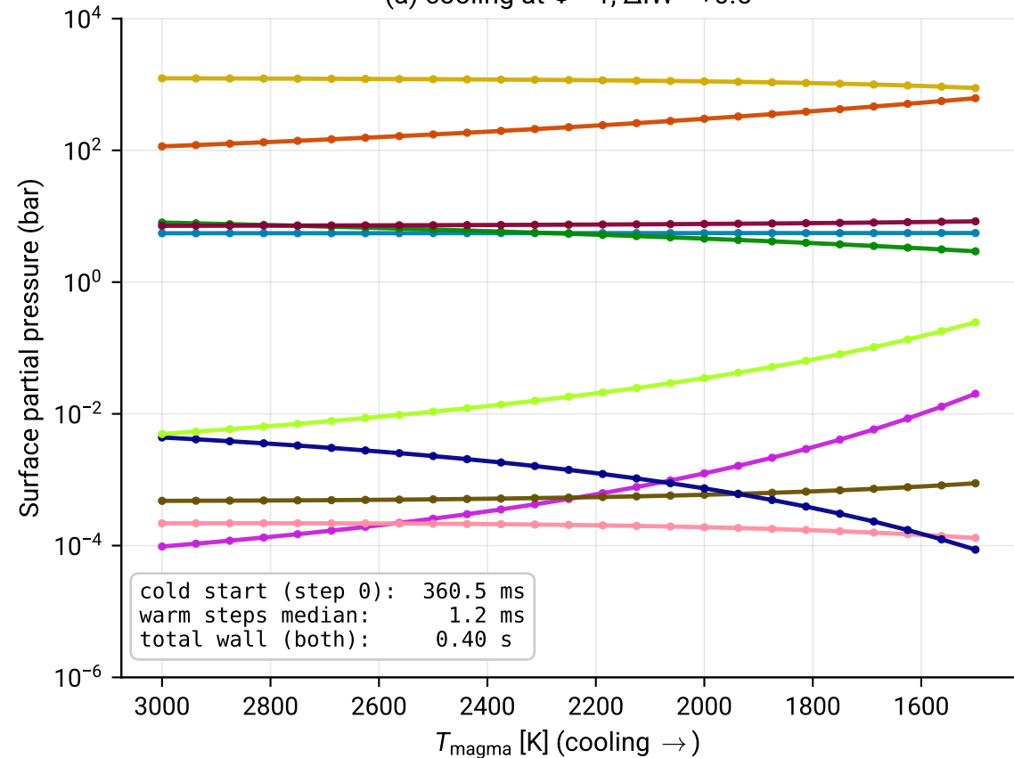
(a) cooling at \Phi = 1 , \Delta IW = +0.5
