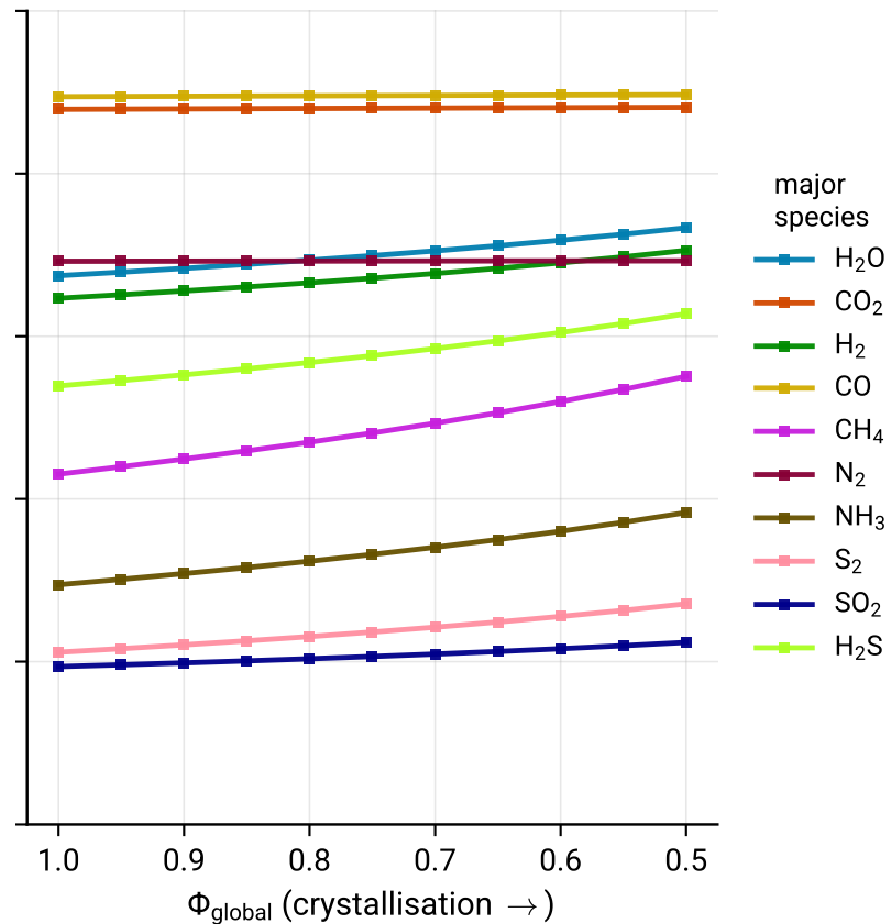
(b) crystallisation at T = 1500 K
