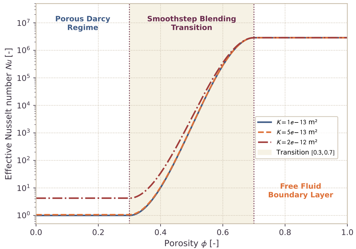
(b) Nusselt Scaling Across Porosity Regimes
