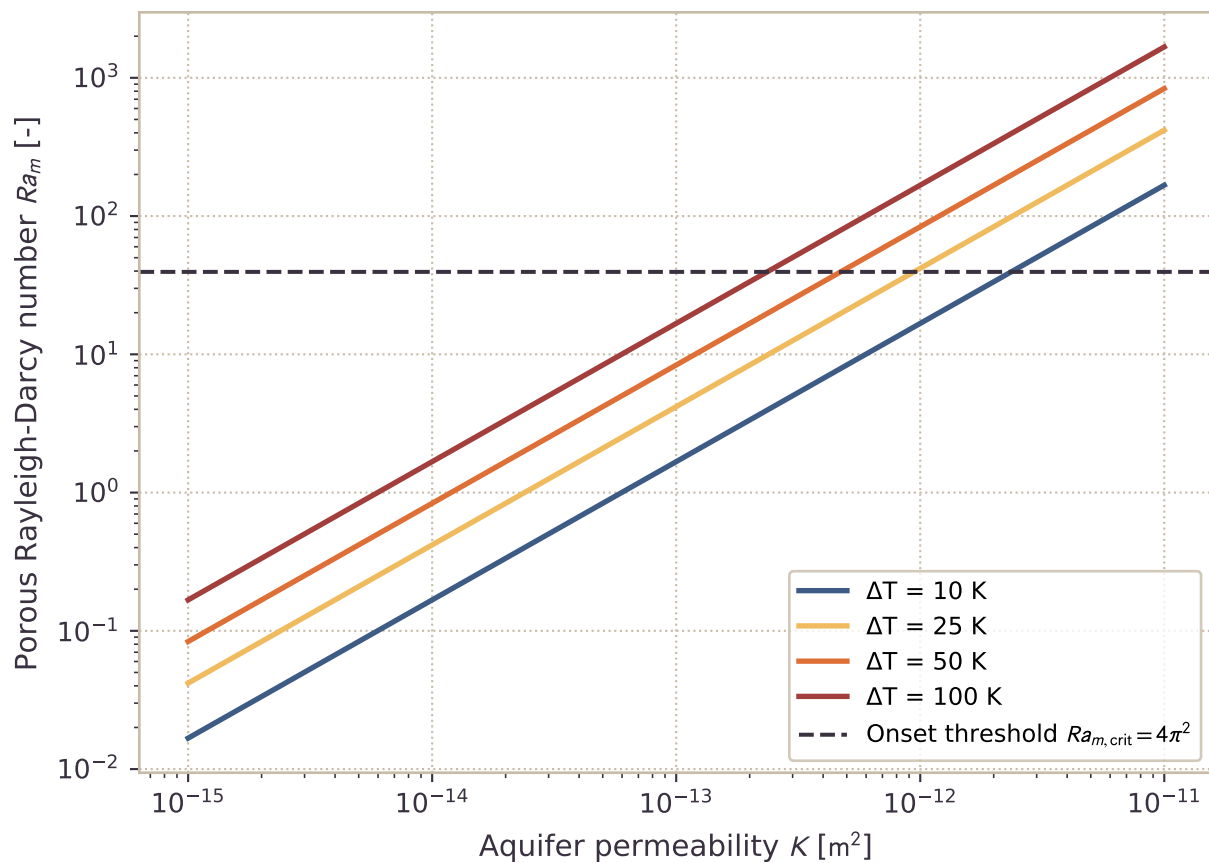
(a) Porous Convection Onset & Scaling
