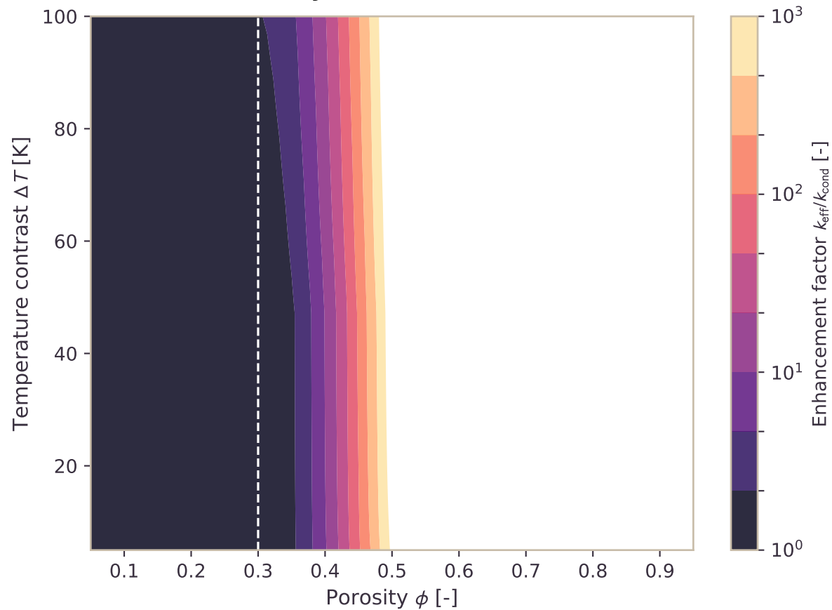
(c) Conductivity Ratio k_{eff}/k_{cond} ( K = 5 \times 10^{-13} m 2 )
