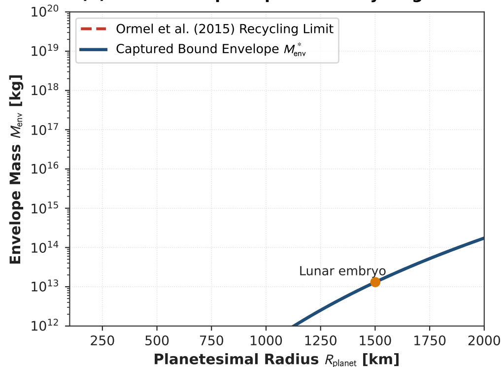
(b) Disk Envelope Capture & Recycling Limit
