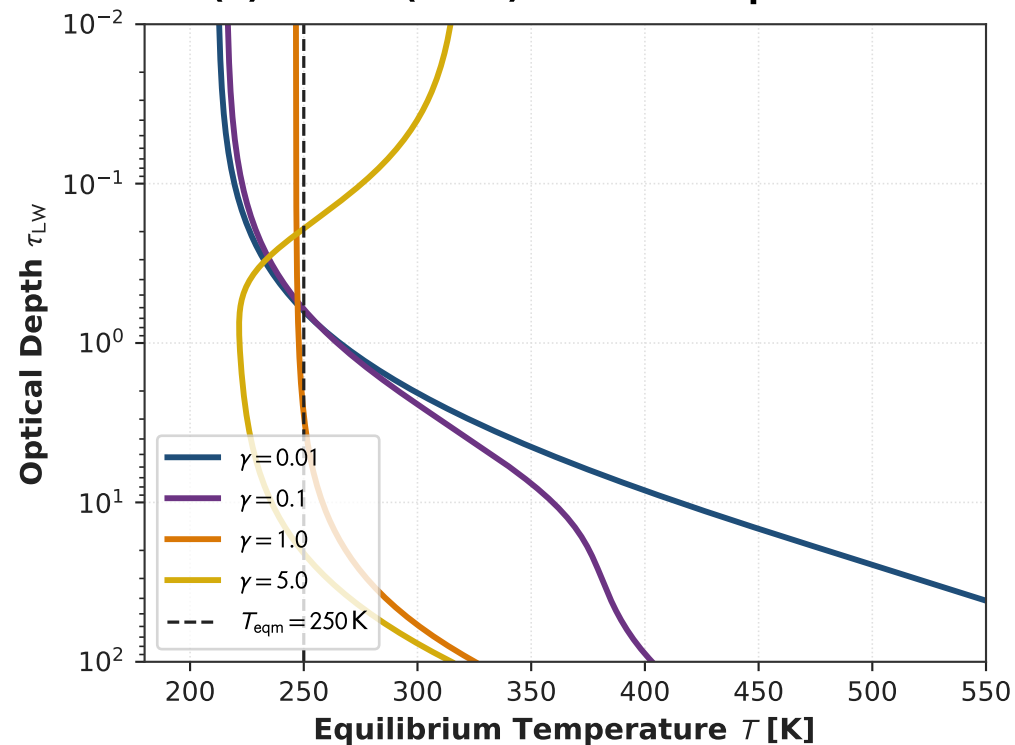
(a) Guillot (2010) Radiative Equilibrium
