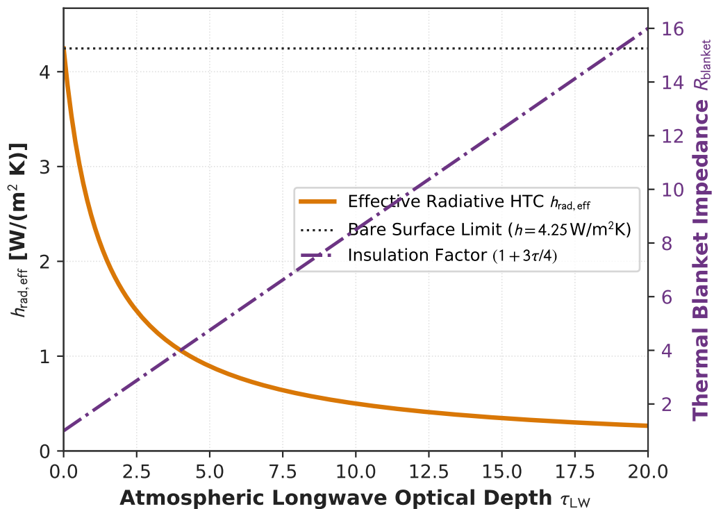
(c) Greenhouse Thermal Blanketing
