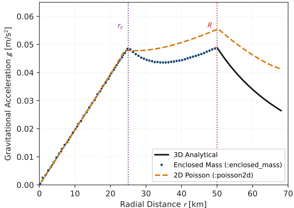
(a) Radial Gravity in Differentiated Planetesimal
