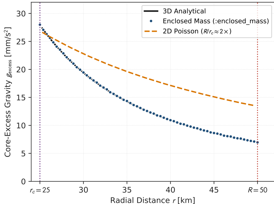
(b) Core-Excess Gravity in Mantle ( r_c \leq r \leq R )
