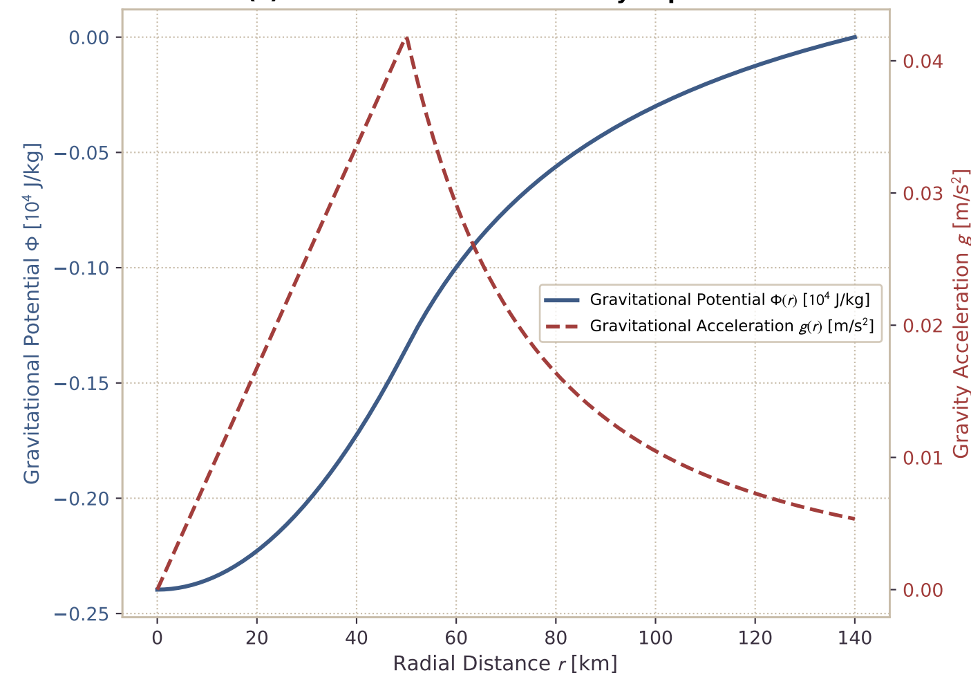
(c) Poisson Potential & Gravity Expansion
