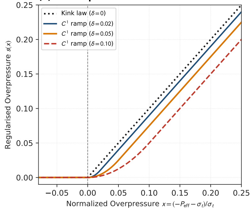
(a) C^1 Overpressure Function
