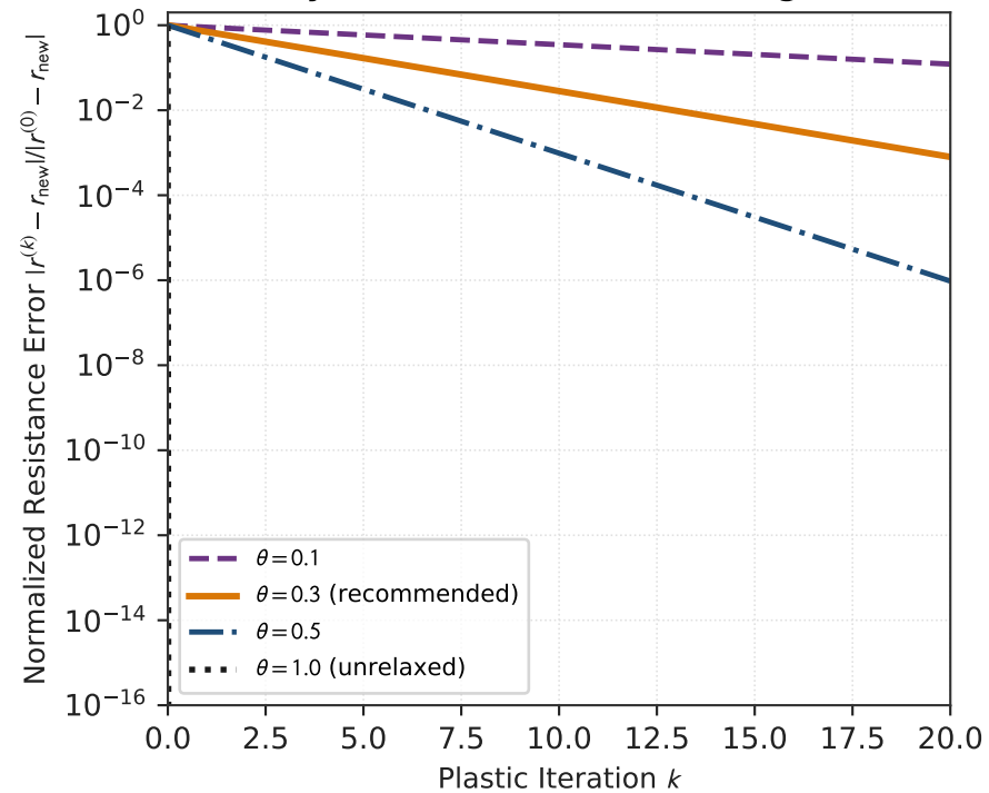
(c) Darcy Under-Relaxation Convergence
