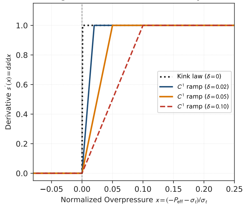
(b) Regularised Derivative Continuity
