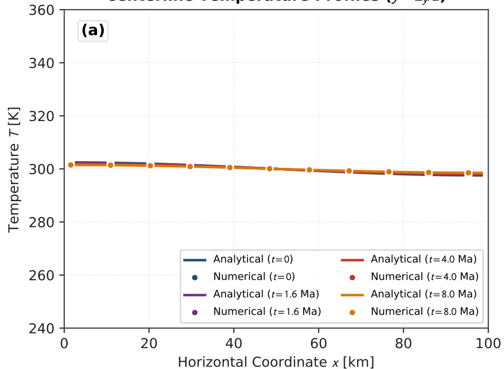
Centerline Temperature Profiles ( y = L_y/2 )
