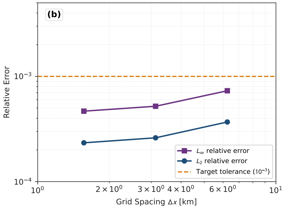
Spatial Grid Convergence ( t=0.1 \tau )
