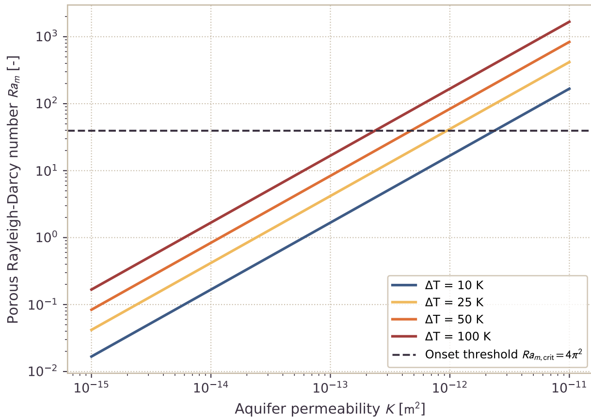
(a) Porous Convection Onset & Scaling
