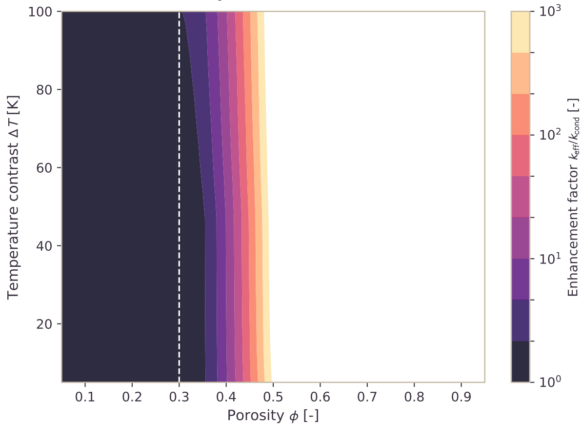
(c) Conductivity Ratio k_{eff}/k_{cond} ( K = 5 \times 10^{-13} m 2 )
