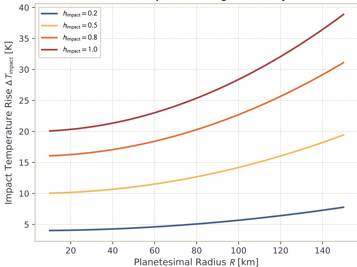
(c) Accretion Impact Heating Thermodynamics
