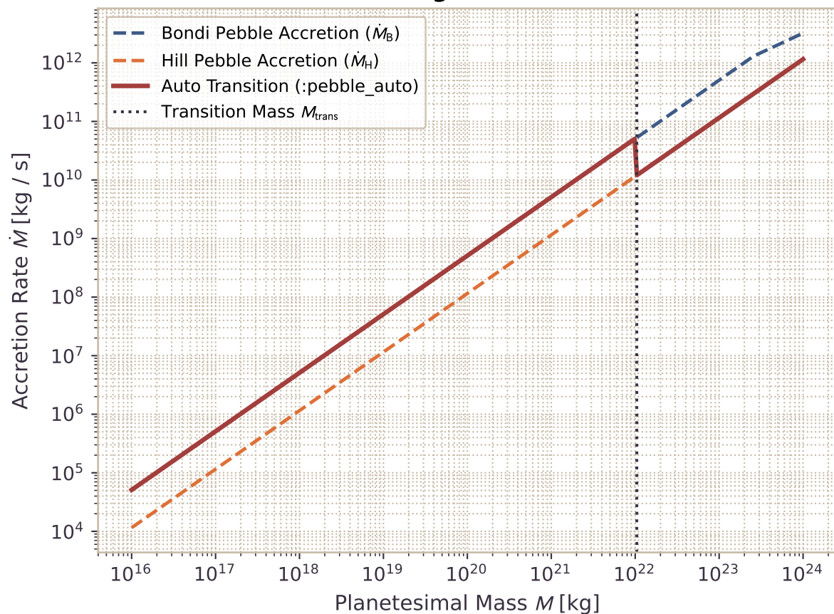
(a) Pebble Accretion Regimes & Bondi-Hill Transition
