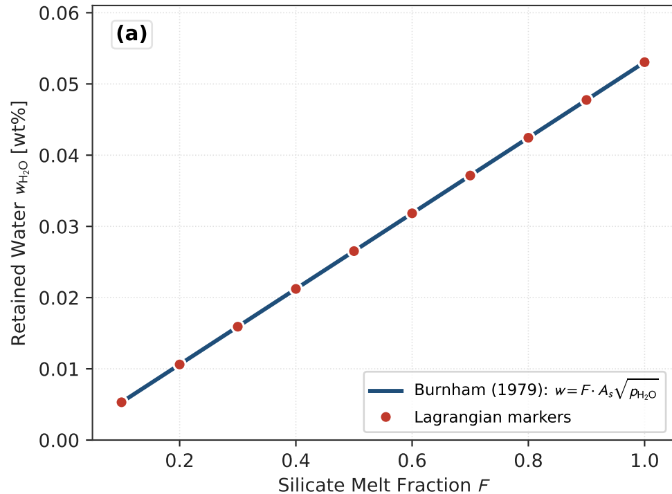
Retained Water vs Melt Fraction
