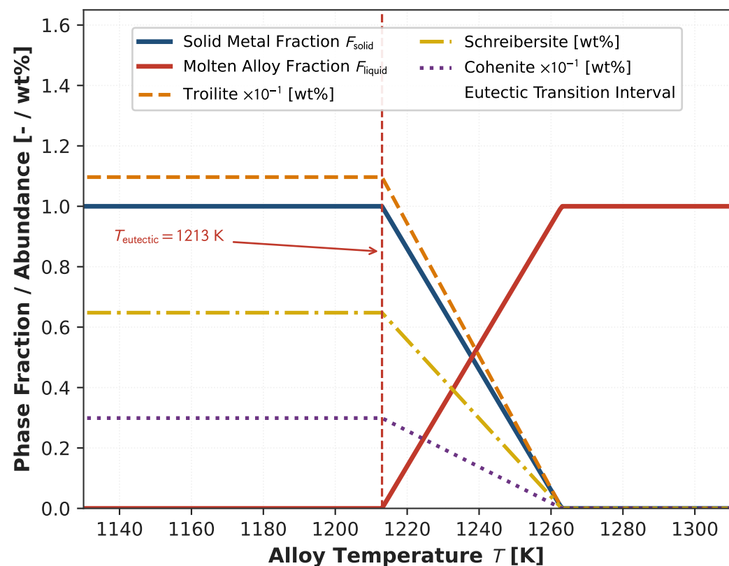
(b) Eutectic Phase Dissolution ( T_{\text{eut}} = 1213 \text{ K} , \Delta T = 50 \text{ K} )
