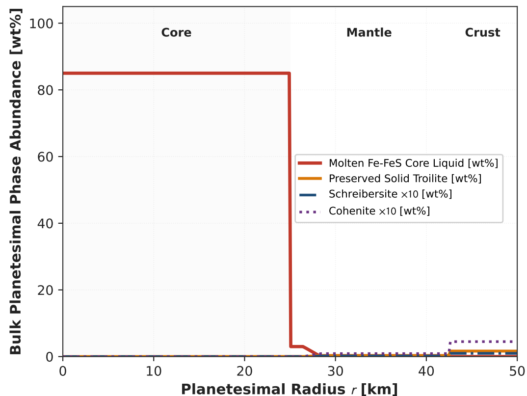
(c) Differentiated Planetary Radial Assemblage
