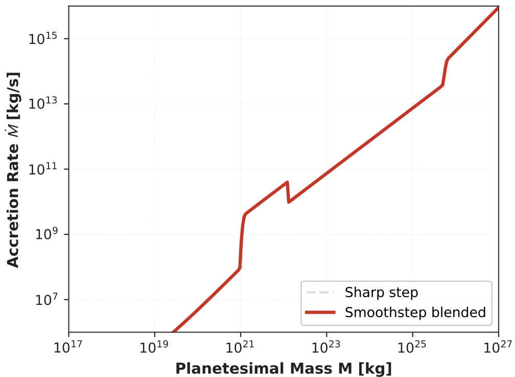
(c) Multi-Stage Accretion Rate Dispatch
