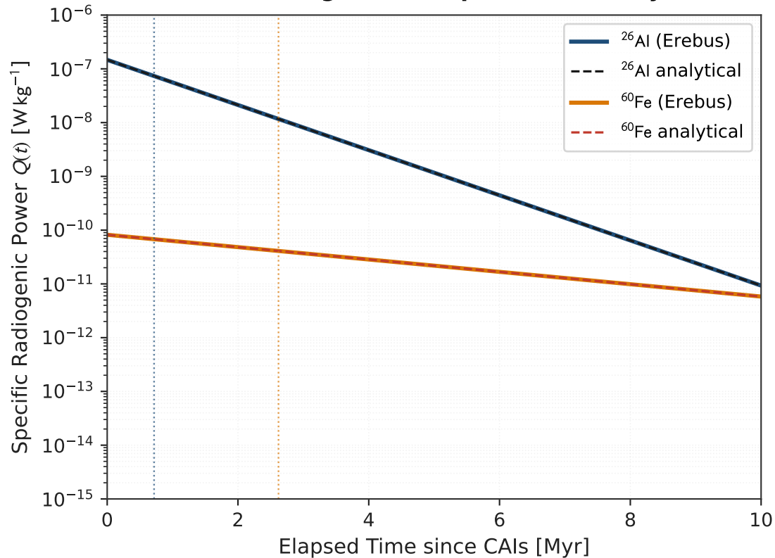
(a) Radiogenic Isotope Power Decay
