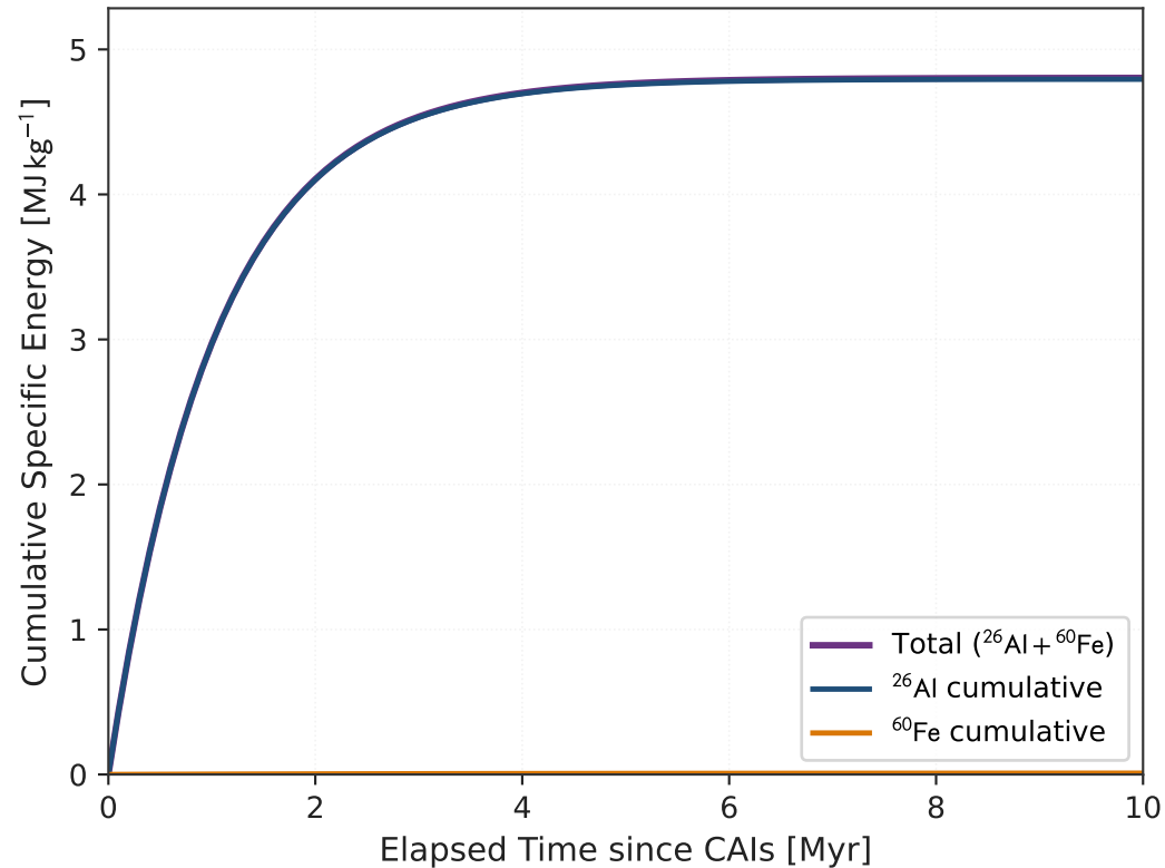
(b) Cumulative Radiogenic Energy Release
