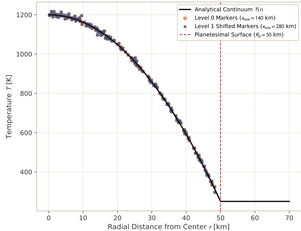
(b) Marker Radial Profile Invariance
