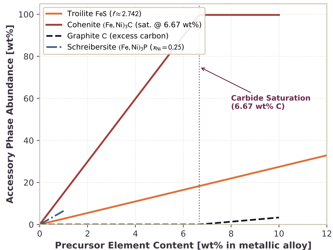
(a) Stoichiometric Accessory Mineral Conversion
