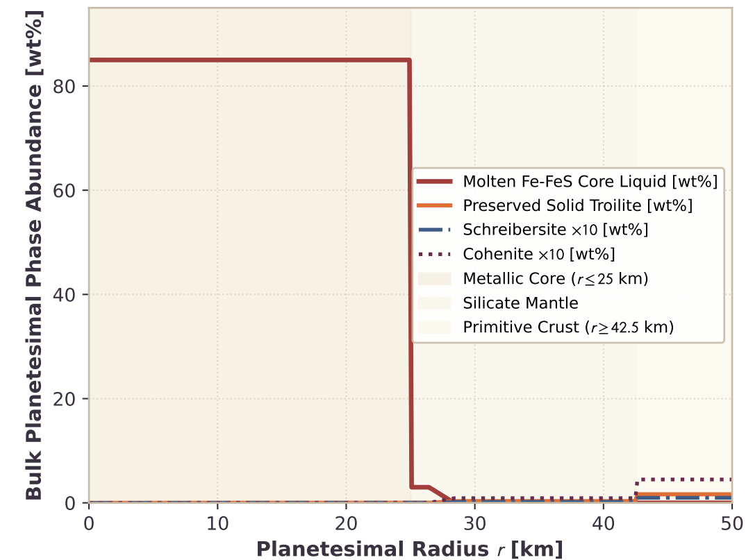
(c) Differentiated Planetesimal Radial Assemblage
