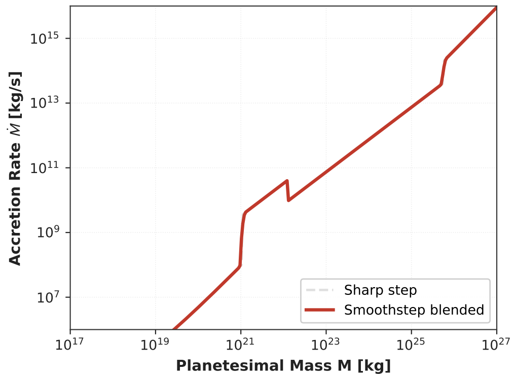
(c) Multi-Stage Accretion Rate Dispatch
