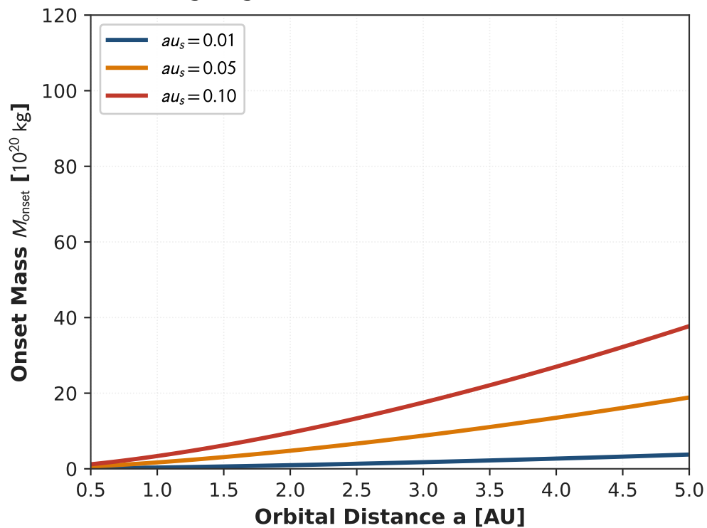
(a) Settling Regime Onset Mass (Visser & Ormel 2016)
