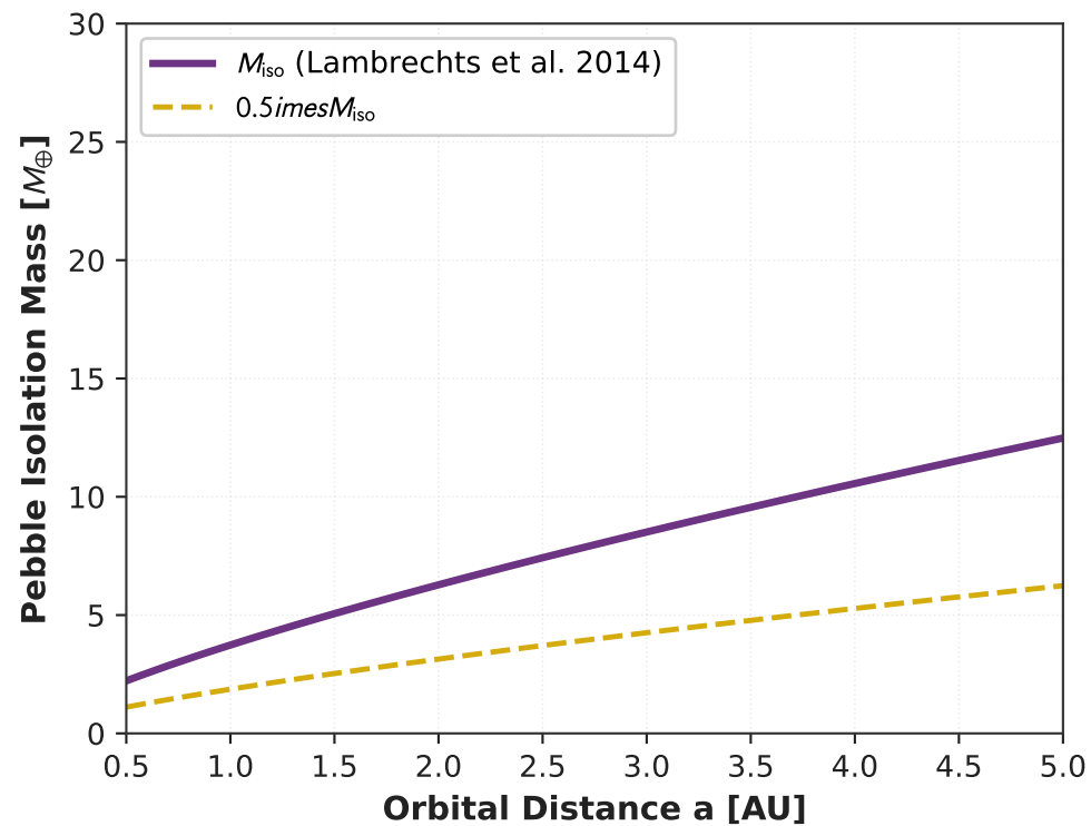
(b) Pebble Isolation Mass (Lambrechts et al. 2014)
