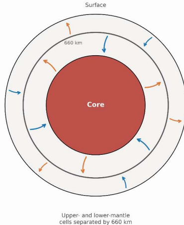
(b) Layered convection
