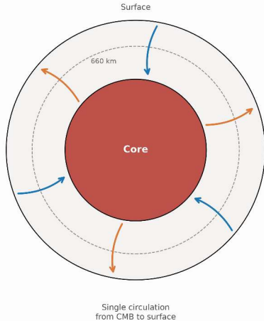
(a) Whole-mantle convection
