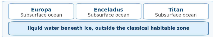
(b) Icy-moon ocean worlds (schematic)
