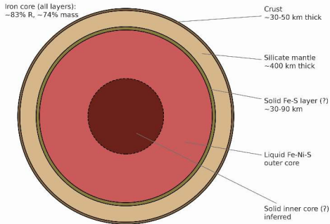
Mercury's interior structure (post-MESSENGER model)
