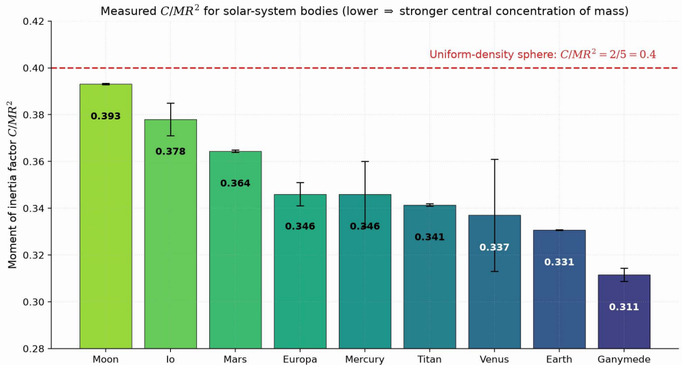
Moment of inertia factors for nine solar-system bodies. Course original; lunar value from Williams et al. (2014).
