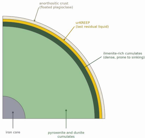
End-state of the lunar magma ocean; thin layers exaggerated. Course figure, after Elkins-Tanton (2012).
