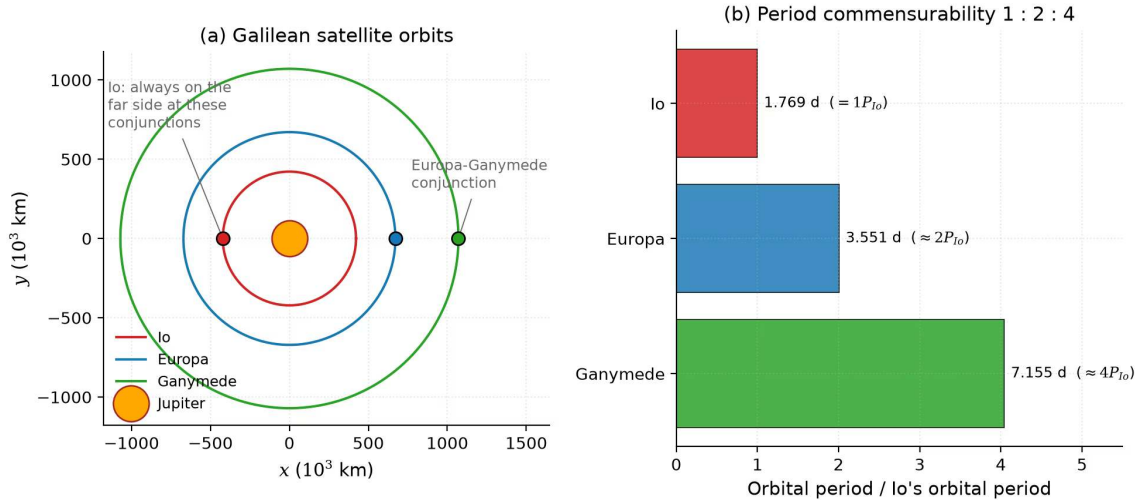
The Laplace resonance of Io, Europa, and Ganymede. Course figure.
