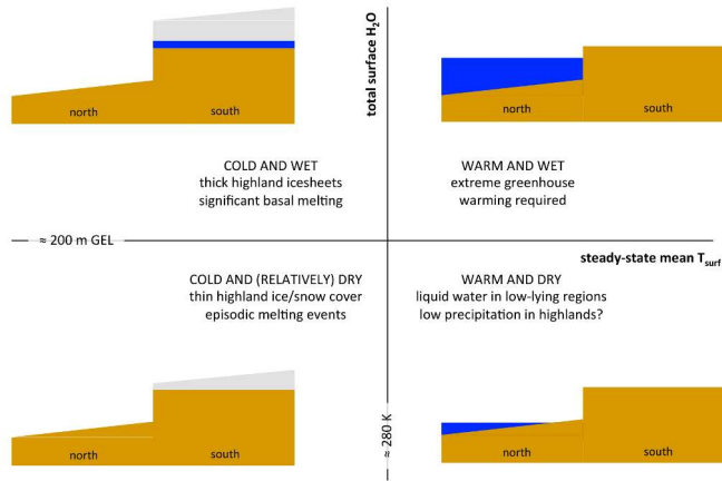
Climate regimes of Mars: H_2O inventory against surface temperature, with cross-sections. Credit: Wordsworth (2016), Fig. 7.
