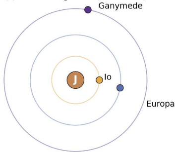
(a) Orbital configuration (not to scale)
