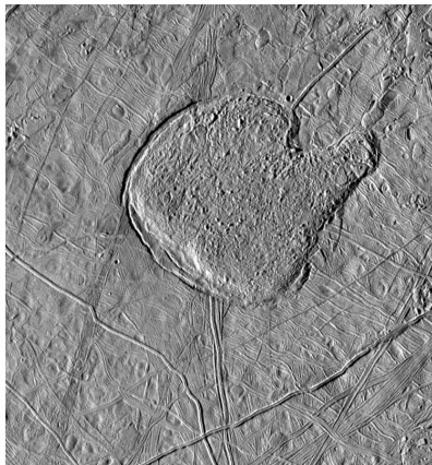
Conamara Chaos on Europa, Galileo (PIA01640). Credit: NASA/JPL-Caltech/ASU.
