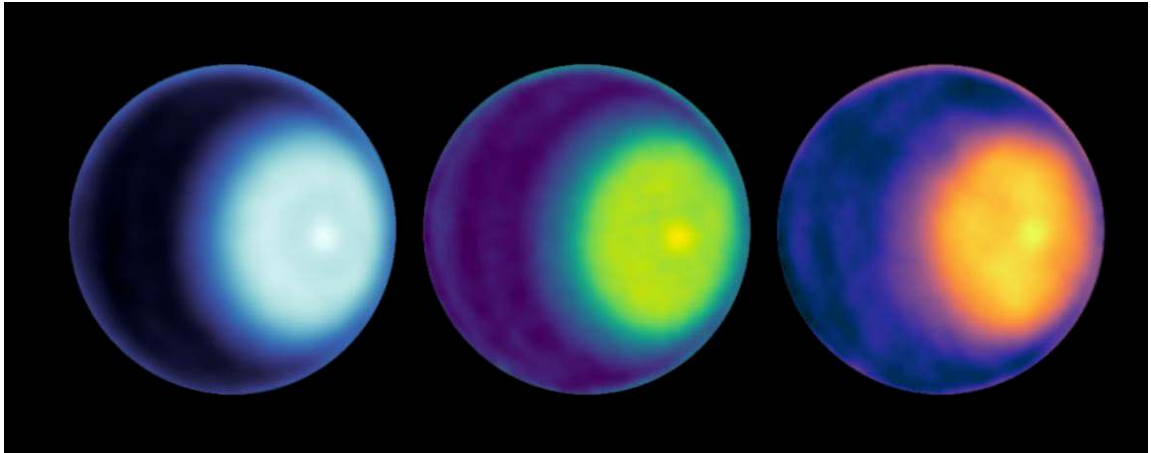
Microwave views of Uranus from the Very Large Array, with the bright north-polar cyclone. Credit: NASA/JPL-Caltech/VLA.
