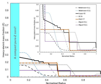
Figure 2. The heavy-element mass fraction in Jupiter as a function of normalized radius. The small panel zooms in to the region beyond the core. The various curves correspond to different published models indicated in the figure. In some models, the innermost ~1% by mass (~10% by radius) of the planet is assumed to be a pure heavy-element region, i.e., a compact core. Others can fit the gravity data without a pure heavy-element core. In all the models, the heavy-element mass fraction in the deep interior is moderate.
