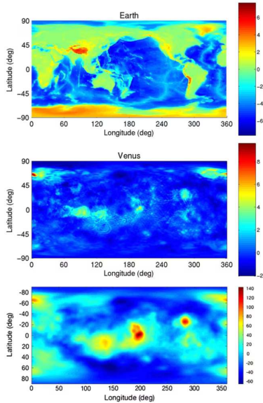
Earth topography, Venus topography, Venus geoid. Smrekar et al. (2018)
