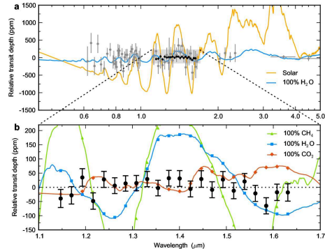
GJ 1214 b: featureless. Kreidberg+ 2014.
