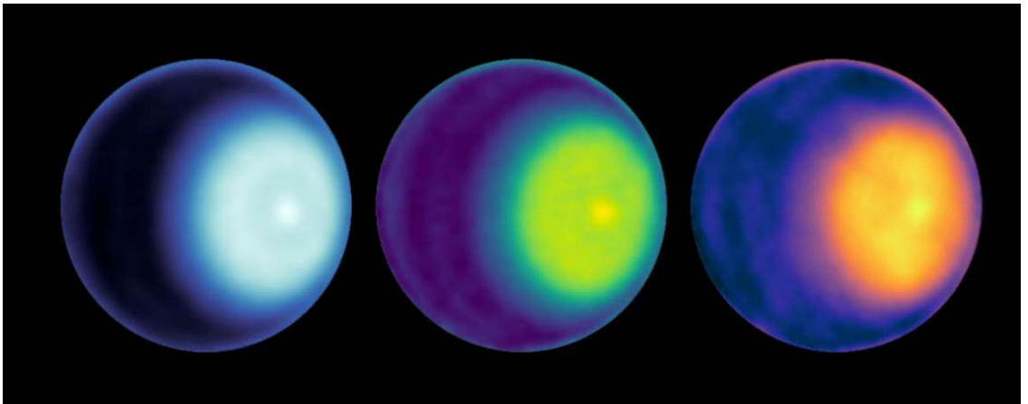
Microwave views of Uranus from the Very Large Array (VLA) with the bright north-polar cyclone. Credit: NASA/JPL-Caltech/VLA.
