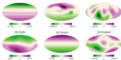
Figure 1. Radial magnetic field at the surfaces of (a) Mercury, (b) Earth, (c) Jupiter, (d) Saturn, (e) Uranus and (f) Neptune. Data taken from [1] for Mercury (with spectral resolution of spherical harmonic degree l \leq 5 ), IGRF-13 coefficients are used for Earth and are available on the IAGA Division V-MOD geomagnetic field modelling website ( l \leq 13 ), [2] for Jupiter ( l \leq 10 ), [3] for Saturn ( l \leq 11 ), [4] for Uranus ( l \leq 4 ) and [5] for Neptune ( l \leq 3 ). The colours represent field intensity, where purple (green) indicates outward (inward) directed field. A mollweide projection is used in which the horizontal lines indicate constant latitude. (Online version in colour.)
