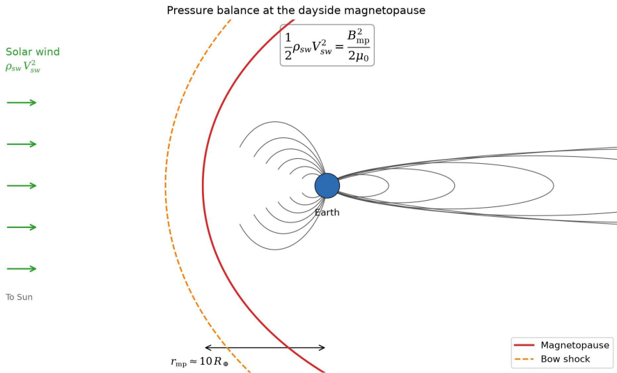
Pressure balance at the dayside magnetopause. Course figure.
