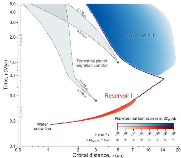
Two planetesimal reservoirs from snow-line migration. Lichtenberg et al. (2021).
