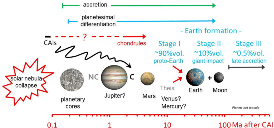
Fig. 5 Summary of timescales for the accretion and differentiation of planetary materials and their connection. Accretion and differentiation timescales after CAI condensation. Mezger et al. (2020).
