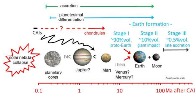
Fig. 5 Summary of timescales for the accretion and differentiation of planetary materials and their connec-
