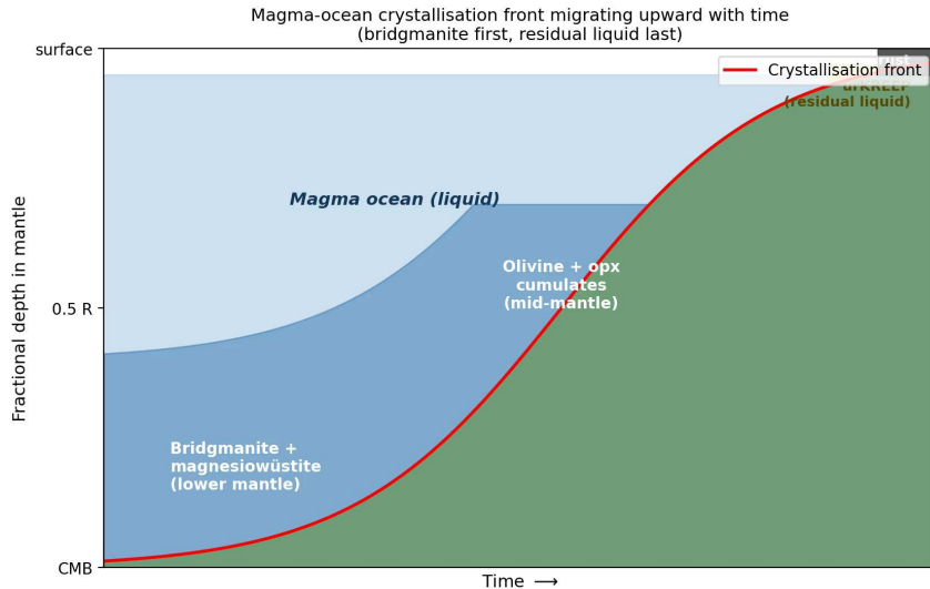
Magma-ocean crystallisation sequence. Elkins-Tanton (2012).
