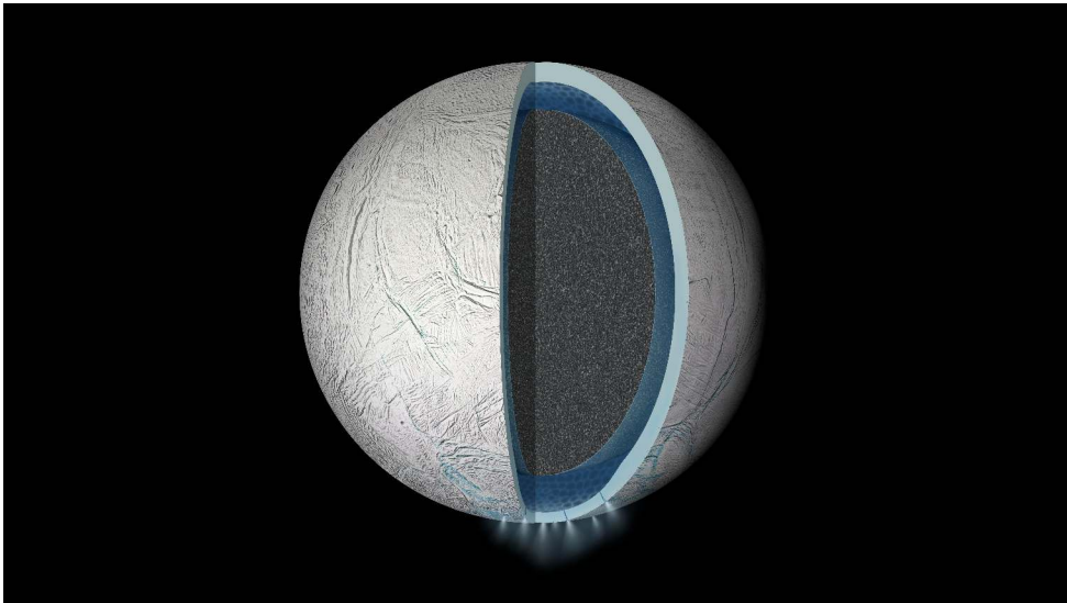
Enceladus in cutaway: ice shell, global ocean, porous rocky core. Credit: NASA/JPL-Caltech (PIA19656).
