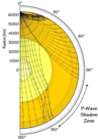
The P-wave shadow zone. Credit: U.S. Geological Survey, public domain.
