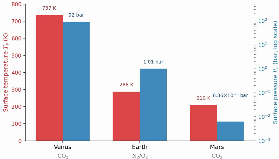
Surface T and P for Venus, Earth, Mars. Data: JPL SSD Planetary Physical Parameters.
