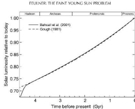
Figure 1. Evolution of solar luminosity over the four geologic eons for the standard solar model described in Bahcall et al. [2001] (solid line) and according to the approximation formula [Gough, 1981] (dashed line) given in equation (1).
