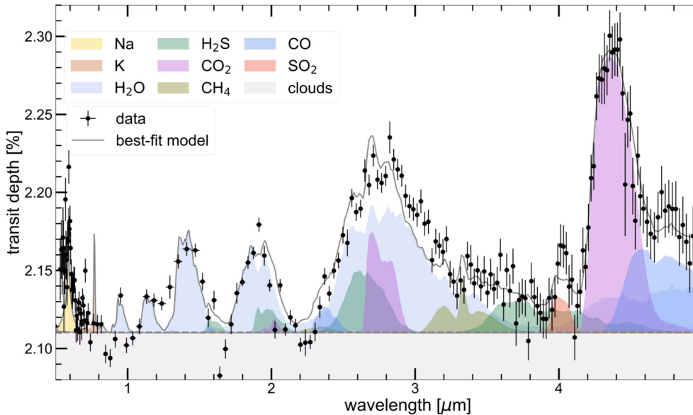
JWST/NIRSpec PRISM transmission spectrum of WASP-39 b: Na, K, \text{H}_2\text{O} , CO, \text{CO}_2 , \text{SO}_2 , \text{CH}_4 , clouds. Rustamkulov+ 2023.
