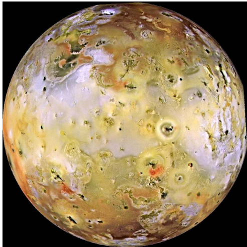
Full-disk view of Jupiter's moon Io from Galileo SSI, showing active sulfur and silicate volcanism powered by tidal dissipation in the Laplace resonance. Credit: NASA/JPL-Caltech/University of Arizona.
