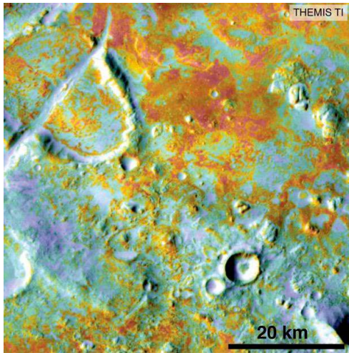
Reflectance spectroscopy of Nili Fossae, Mars: THEMIS thermal inertia (left) and CRISM mineralogy (right) revealing Mg-carbonates (green), olivine sands (yellow), and basalt (blue). Scale bars: 20 km. Credit: NASA/JPL-Caltech/ASU/JHU APL.
