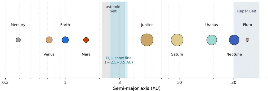
Architecture of the Solar System on a logarithmic semi-major-axis scale. Course-original figure; data: NSSDC Planetary Fact Sheet.
