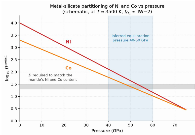
Metal-silicate partition coefficients versus pressure. Course figure, after Siebert et al. (2013).
