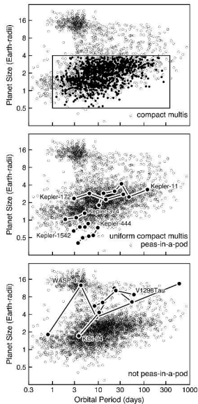
Transiting census; box and filled circles are compact multis (top), five uniform ones (middle), three non-uniform (bottom). Weiss et al. (2023, PPVII).
