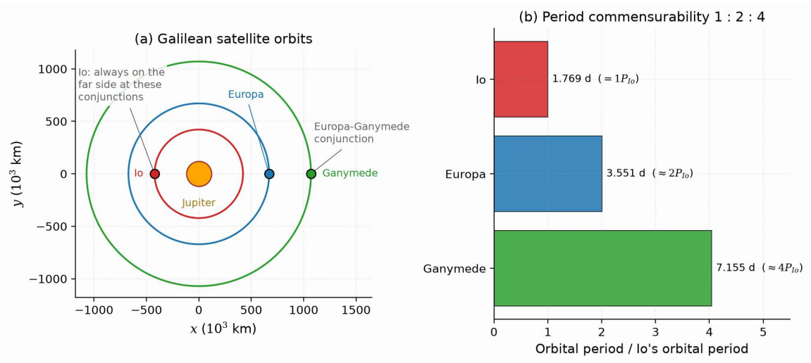
The Laplace resonance of Io, Europa, and Ganymede. Course-original figure.
