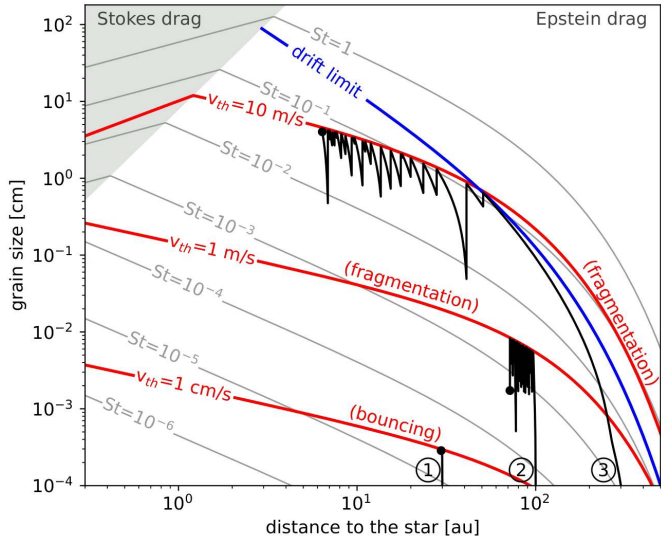
Maximum grain size vs orbital distance in a standard disk model. Reproduced from Drążkowska et al. (2023), Fig. 4.
