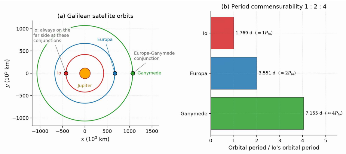
The Laplace resonance of Io, Europa, and Ganymede. Course figure.
