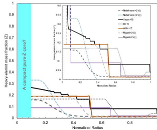
Figure 2. The heavy-element mass fraction as a function of normalized radius. The small panel zooms in to the innermost region. The various lines correspond to different published models indicated in the figure. In some models, the innermost ~1% by mass (~10% by radius) of the planet is assumed to be a pure heavy-element region, i.e., a compact core. In all the models, the heavy-element mass fraction in the deep interior is moderate.
