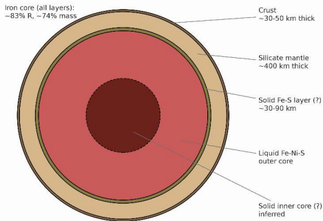
Mercury's interior structure (post-MESSENGER model)
