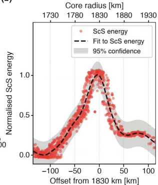
(a) Marsquake S0173a and the six-event stack against time from ScS; (b) ScS energy against core radius, normalised to the fit. Adapted from Stähler et al. (2021).
