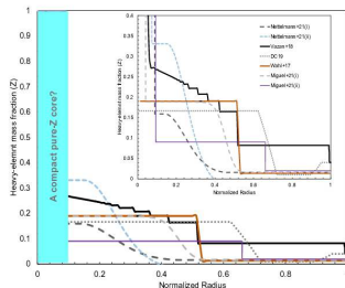
Figure 2. The heavy-element mass fraction as a function of normalized radius for Jupiter. The small panel zooms in to the region beyond the core. The various lines correspond to different published models indicated in the figure. In some models, the innermost ~1% by mass (~10% by radius) of the planet is assumed to be a pure heavy-element region, i.e., a compact core. In other models, others can fit the gravity data without a pure heavy-element core. In all the models, the heavy-element mass fraction in the deep interior is moderate.
