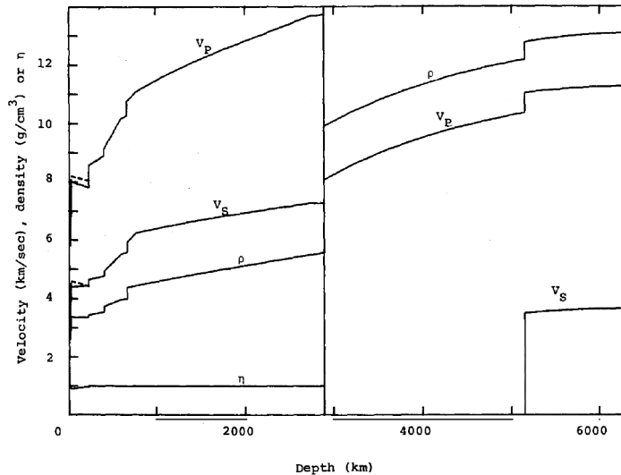
PREM radial profiles of wave speeds, density, and anisotropy. Credit: Dziewonski & Anderson (1981), Fig. 8.
