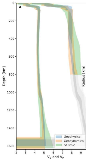
Mars v_p and v_s profiles from InSight. Credit: Stähler et al. (2021), Fig. 2A.
