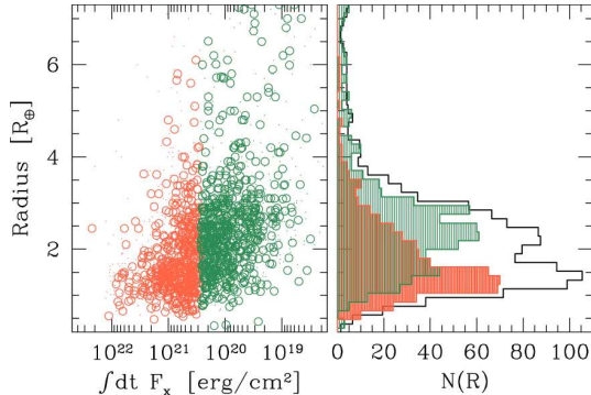
Predicted radius valley
