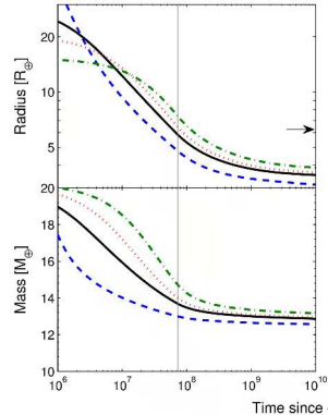
Time evolution of radius + mass
