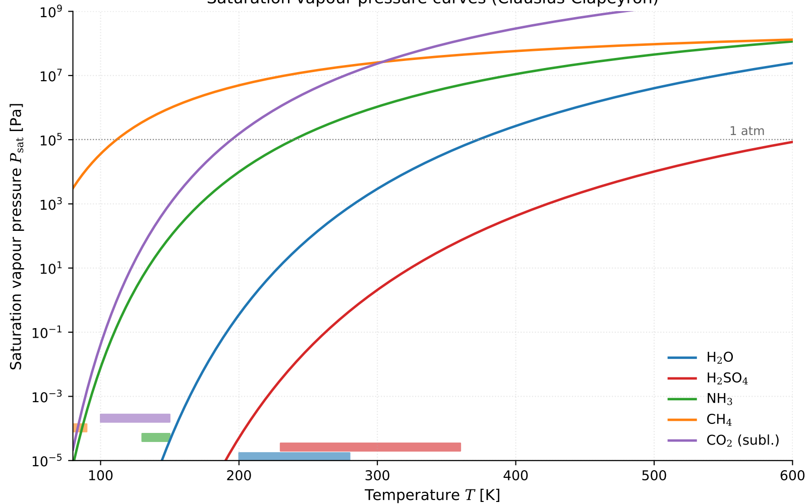
Saturation vapour pressure curves (Clausius-Clapeyron)
